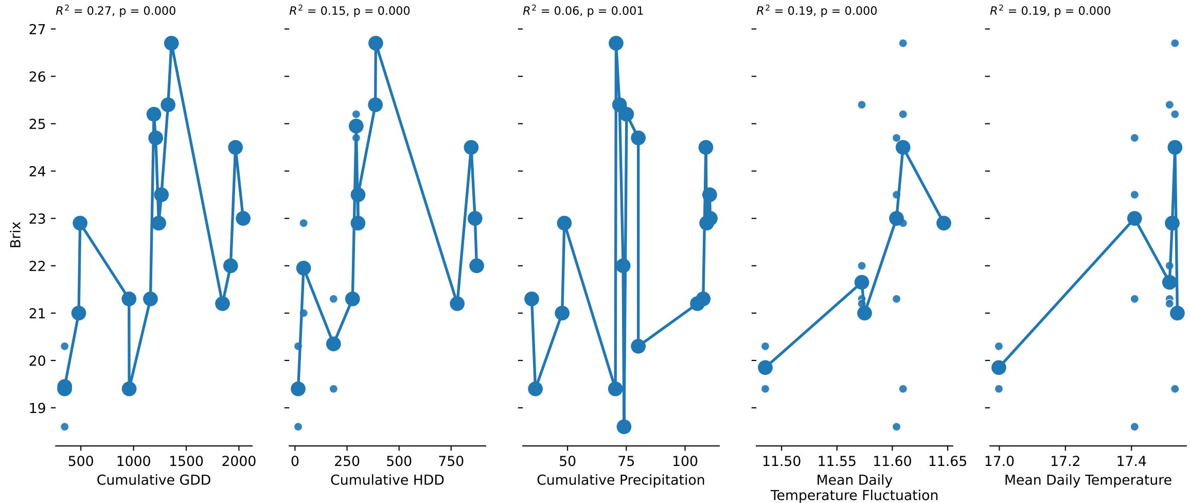
Climate impacts on Brix for Marquette, 2019
